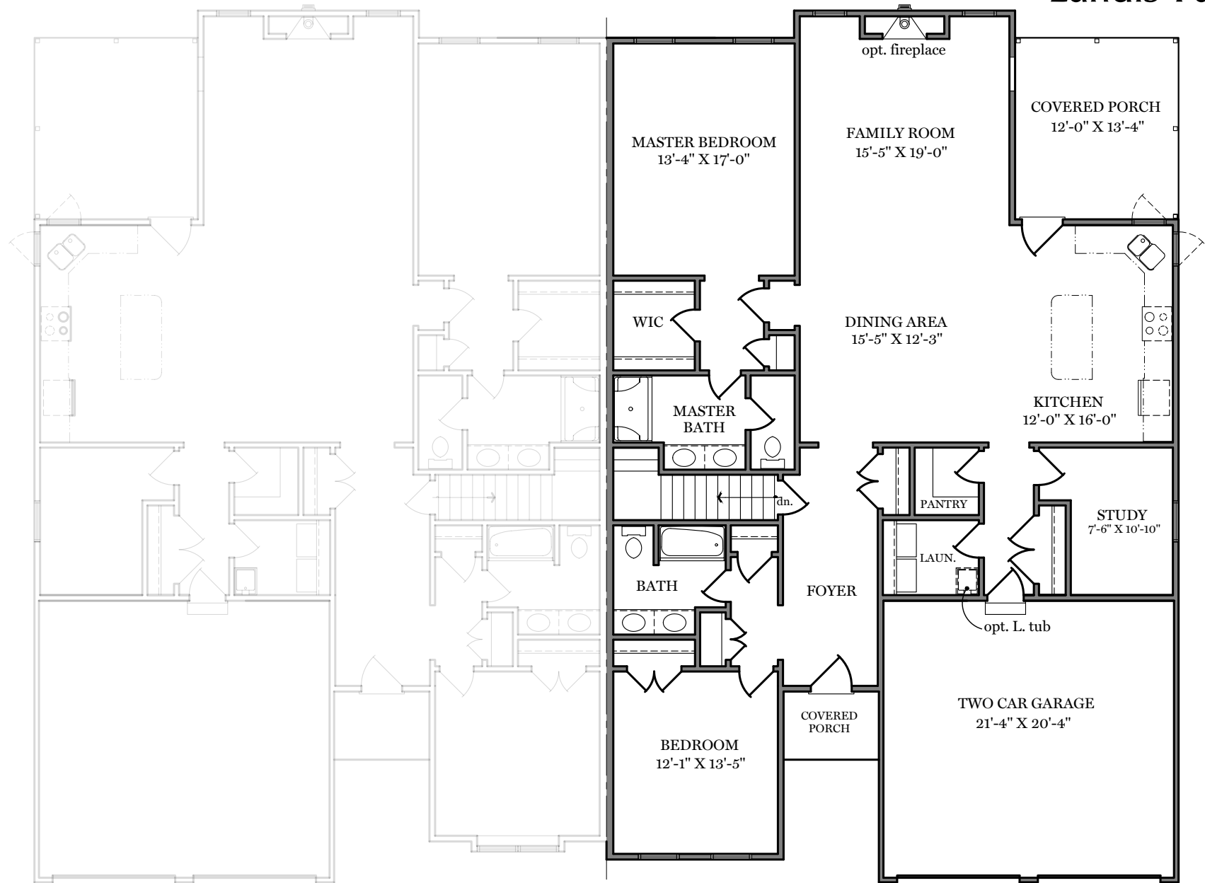
First Floor Plan - 1,904 sf "CORIANDER II" (full basement option shown)
