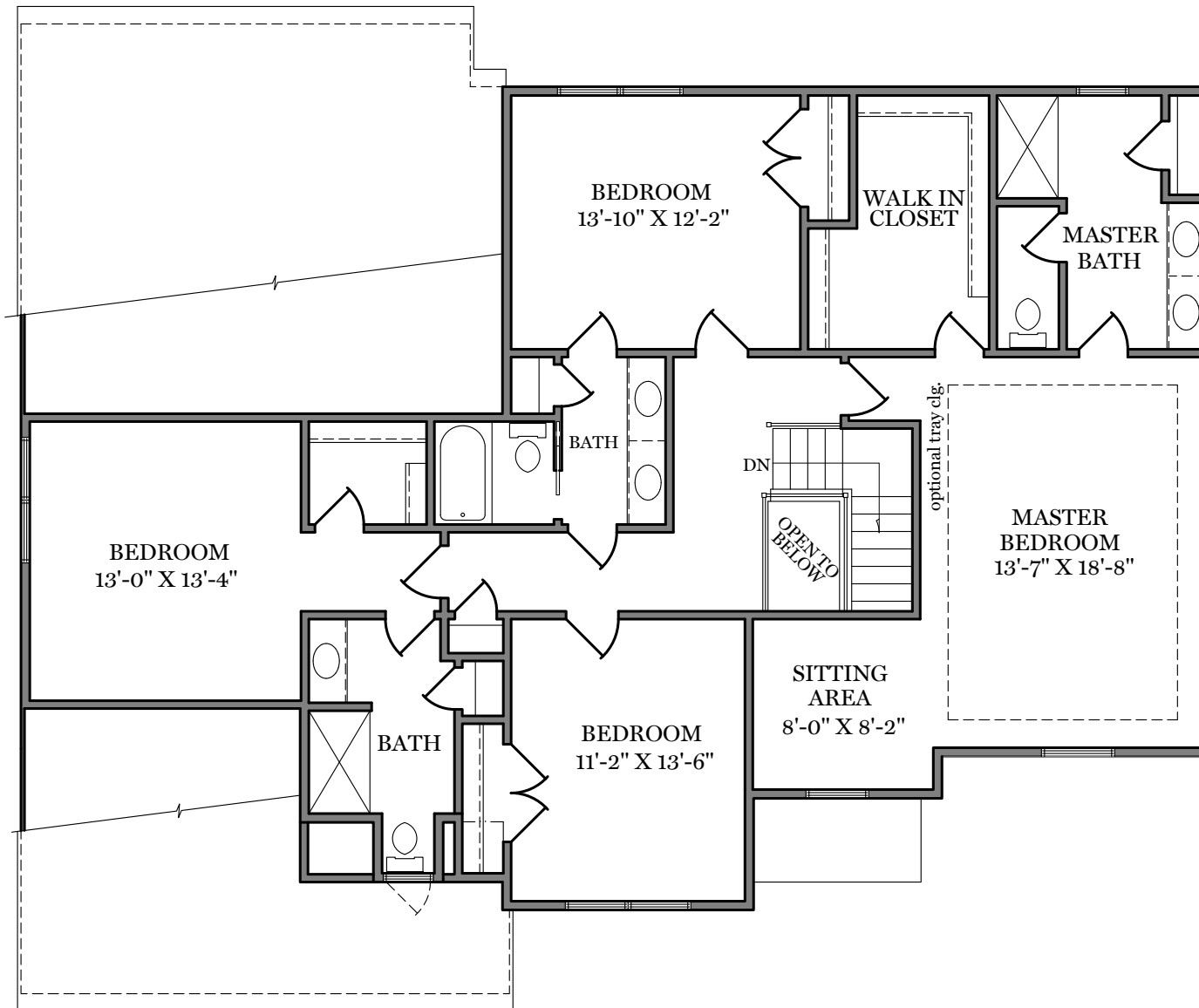
Second Floor Plan - 1,586 sf "MAGNOLIA"
